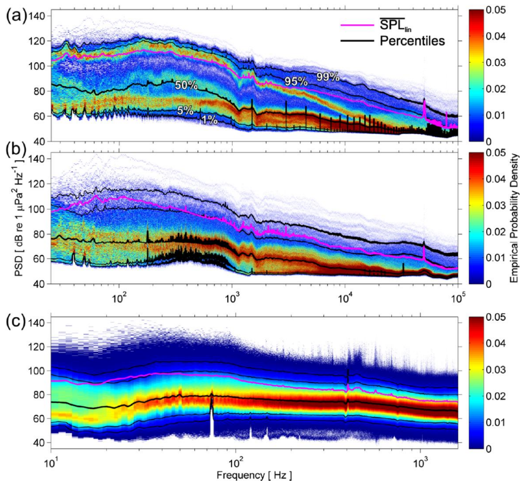
Figure 3. Spectra from Merchant et al. (2013) illustrating the percentile metrics and the arithmetic mean (here termed SPL_{lin} ), together with the underlying noise level distribution (spectral probability density). (a) and (b) are from the Moray Firth in Scotland, (c) is from a shipping lane, the Strait of Georgia in British Columbia.
