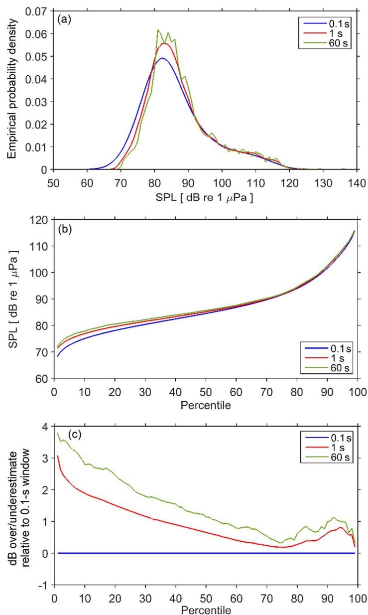
Figure 4. Comparison of noise level statistics in the 1/3-octave band centered at 125 Hz measured over a one-week period using different snapshot windows: 0.1 s, 1 s, and 60 s. (a) Empirical probability densities; (b) Percentile values; (c) Deviation of each percentile from 0.1-s values.
