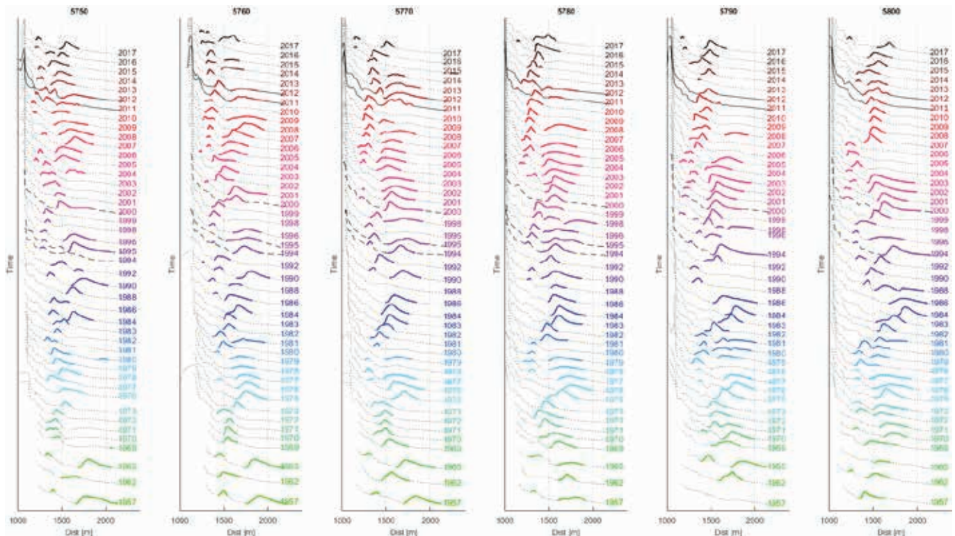
Figure 75 Time stack plot of the Skodbjerg west coast profiles which have a spacing of 1000 meters from 1957 to 2017. The profiles are organized left to right from the north to the south. The long-term bar migration is illustrated by colouring the bar shape. Furthermore, years with nourishment are shown: No nourishment since last nourishment (grey profile), Beach nourishment (dashed profile) and shoreface nourishments (black profile).
