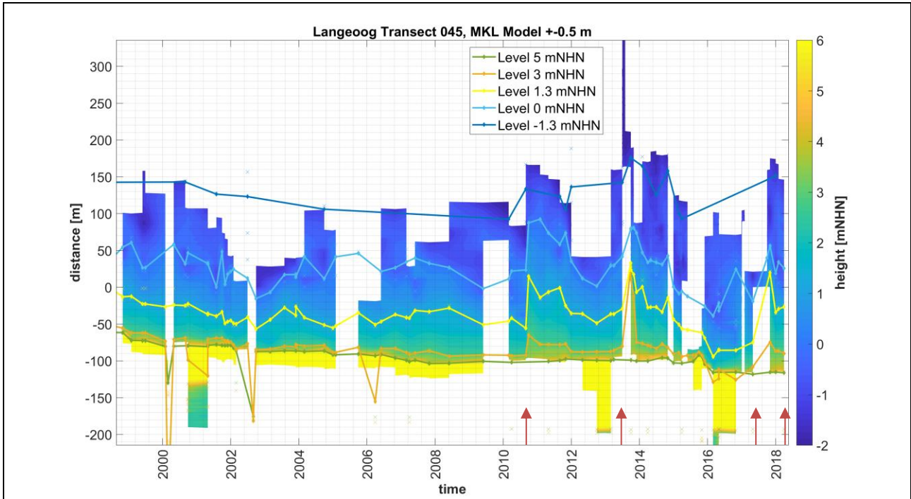
Figure 24 Transect 45. Arrows indicate nourishments.
