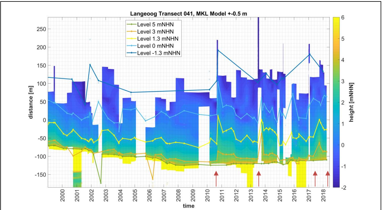
Figure 23 Transect 41. Arrows indicate nourishments.
