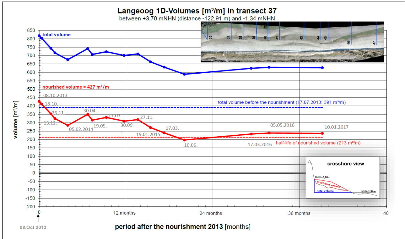
Figure 26 1D-Volumes in transect 37 for the nourishment 2013
