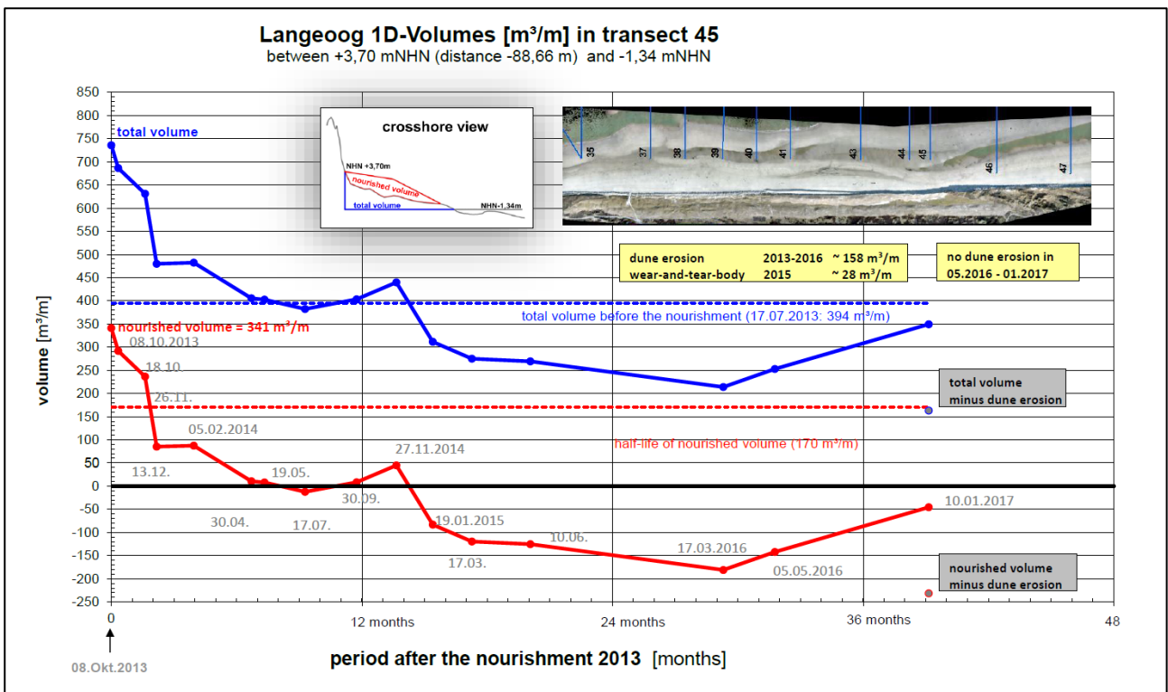
Figure 28 1D-Volumes in transect 45 for the nourishment 2013. There was dune erosion in the period of 2013 to 2016. This sand from the dune moved into the selected area for calculating the 1D-Volume. In the figure the lines represent the calculated volume. The points represent the calculated volume minus the sand of the dune erosion.
