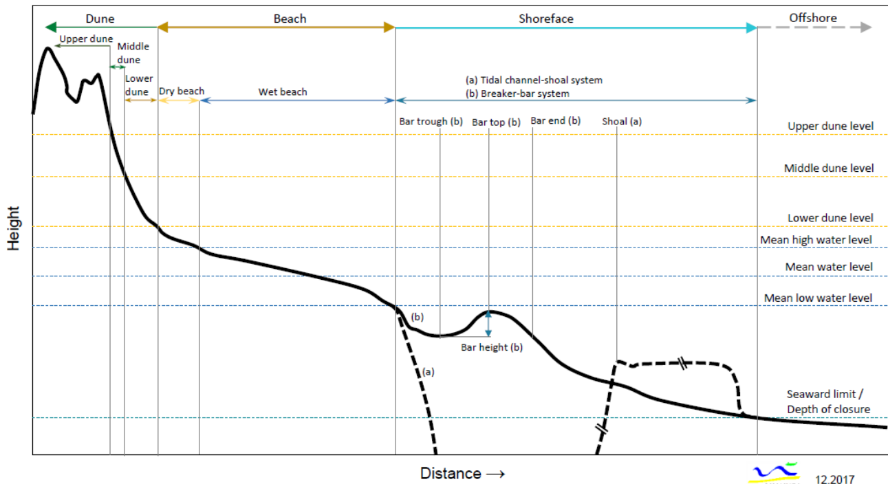
Figure 14 - General terminology used to describe the coastal profile. On the vertical axis various levels in the profile are shown. The horizontal axis shows different morphological zones in the profile.
