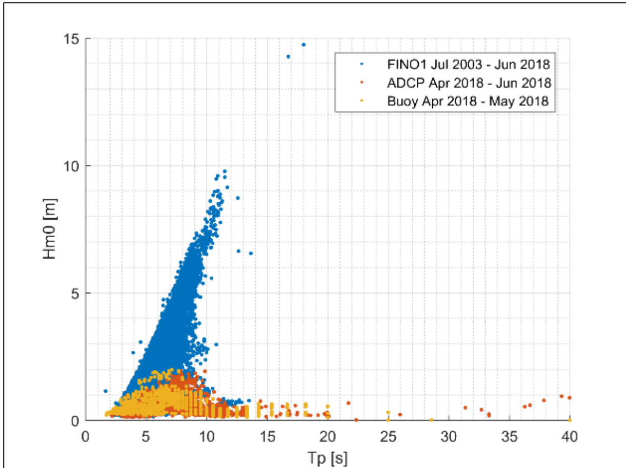
Figure 16 Different measurement platforms to compare results. IMPORTANT: Different time periods in this figure.
