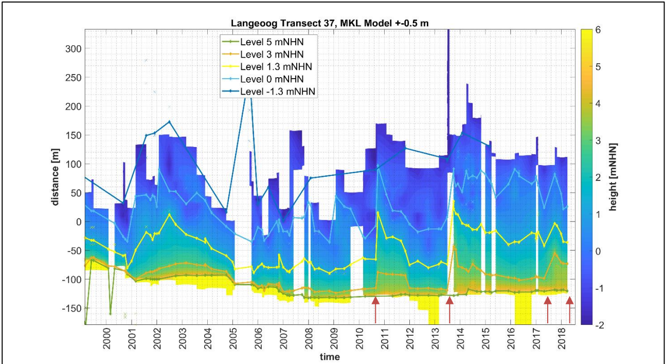
Figure 22 Transect 37. Arrows indicate nourishments.
