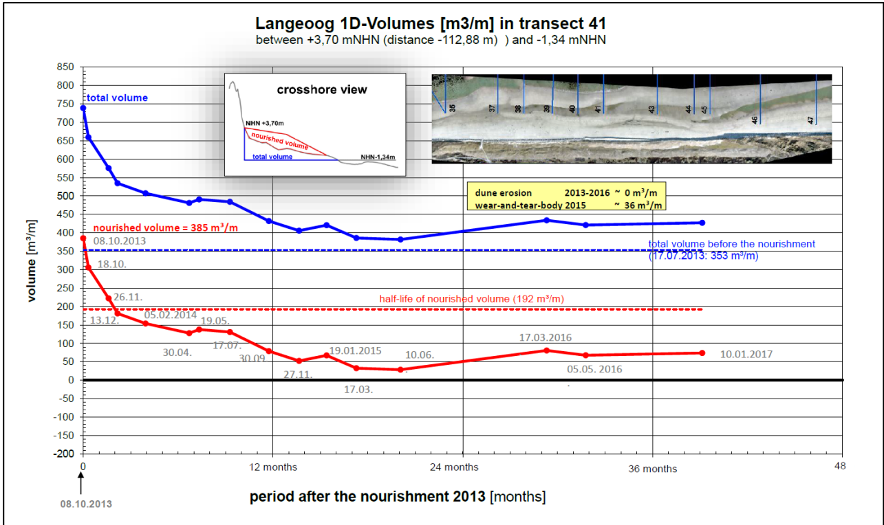
Figure 27 1D-Volumes in transect 41 for the nourishment 2013.
