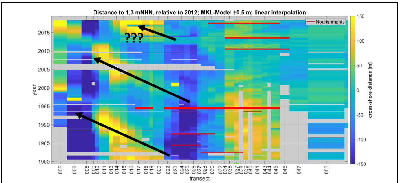
Figure 5 Time Distance Diagram of the main transects of Langeoog. See Figure 4 for the location of transects. Arrows are set manually to indicate sand migrating on the western head of the island from north to south.
