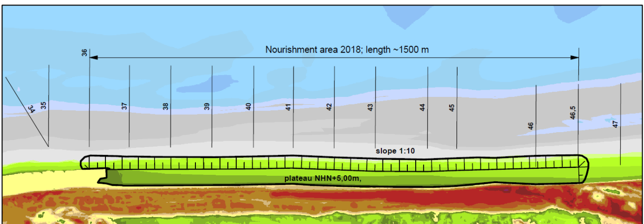
Figure 13 Plateau-design of the nourishment 2018
