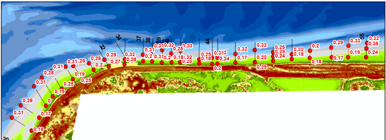
Figure 18 Spatial distribution of d_{50} mean grain size parameter [mm], measured before the nourishment 2017
