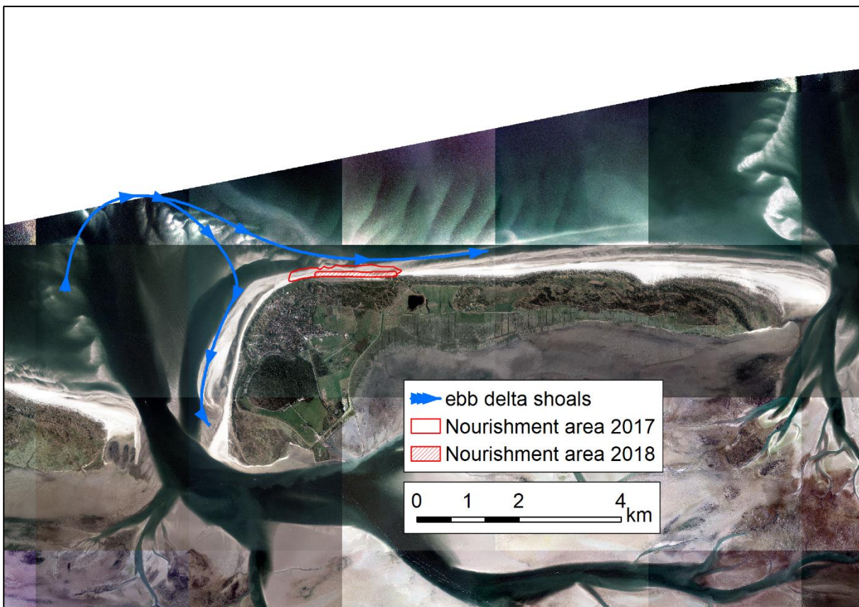
Figure 3 Littoral drift and ebb delta of Accumer Ee (tidal inlet between Baltrum and Langeoog)
