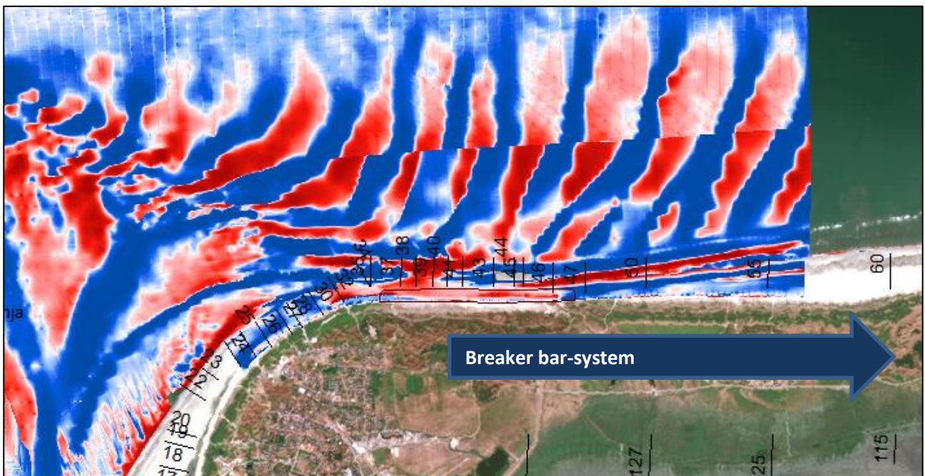
Figure 19 Qualitative differential map of two bathymetry measurements. Colors are oversaturated for better understanding.
