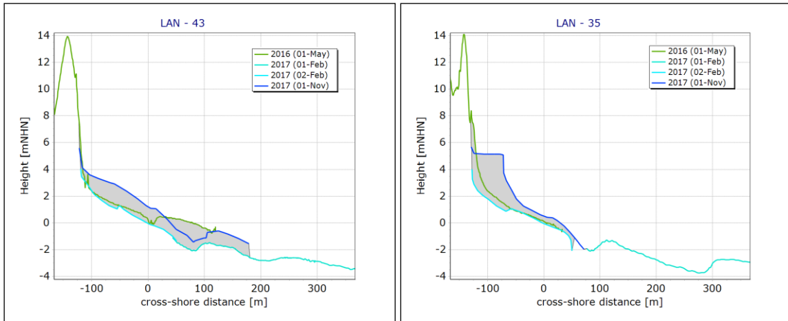
Figure 11 Design of the nourishment 2017 Western part is designed as a plateau (transect 35), the eastern part has a more flat slope (transect 43).
