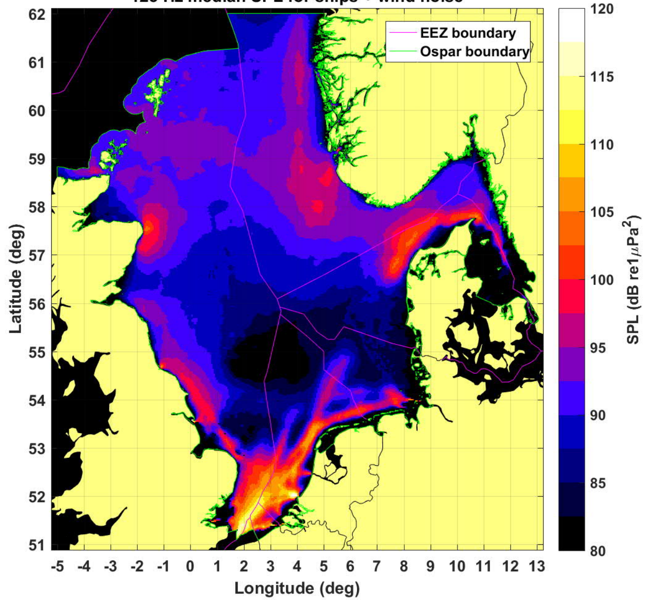
125 Hz median SPL for ships + wind noise
