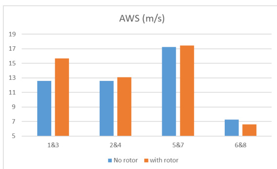
Figure 13a. Apparent wind speed for pairs of runs with and without rotor.
